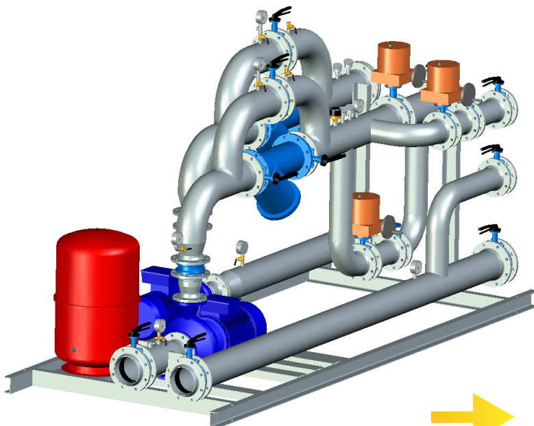
3D view
