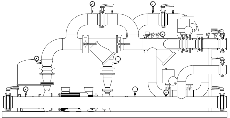
2D drawing
